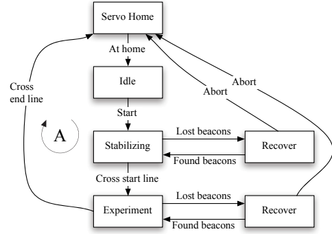
Fig. 4. Illustration of state machine used for automated gait optimization. A trial is considered successful if loop A occurs. Other loops occur if the robot loses sight of the beacons for longer then a predefined time or a critical situation occurs. Only critical situations require human intervention, in general the robot is able to recover by rotating in place until the beacons appear in the field of view of the onboard camera.
